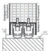
2 x RS1 double joint escamotable
